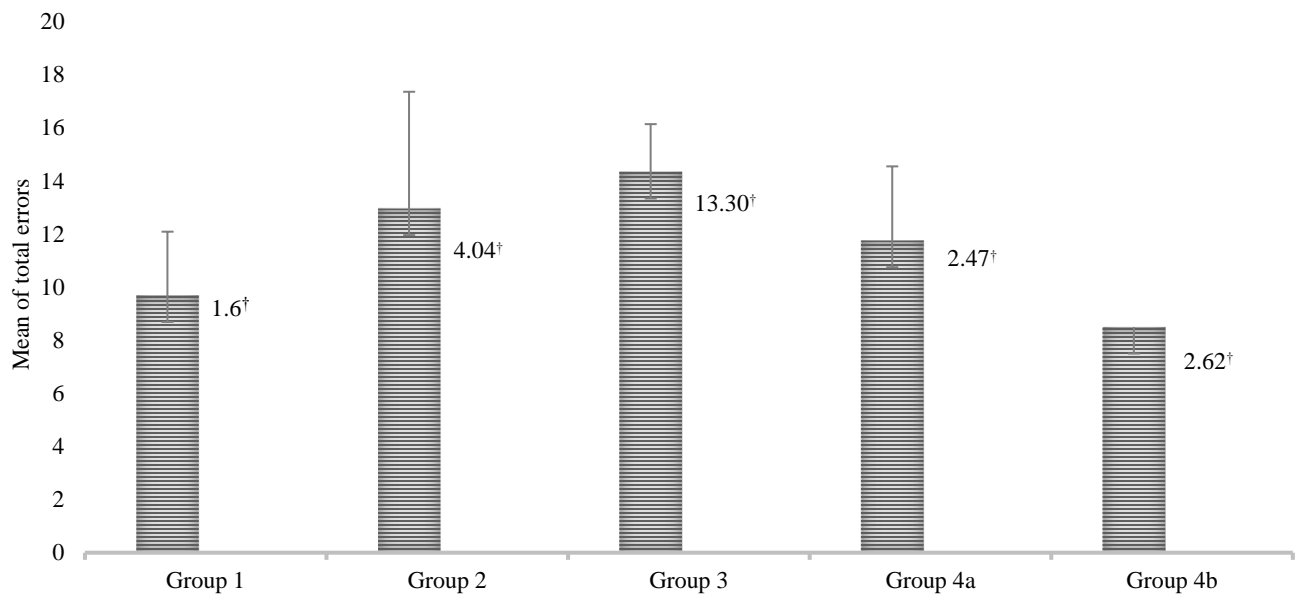
Fig. 2. Shows the mean values and standard deviation of total error in spatial working memory task among all groups, † – mean value of TSH, group 1 – controls, group 2 – newly diagnosed cases, group 3 – patients with elevated TSH levels (ongoing LT-4), group 4a – euthyroid (on LT-4 for 1 or more than one year but less than 5 years), group 4b – euthyroid (on LT-4 for 10 or more years)
